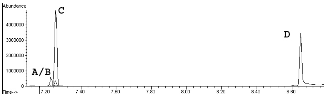
Figure 9. Gas chromatogram for confirmation of norfluoxetine (B), norketamine (C), desmethyldoxepin (D) with internal standard (A).
