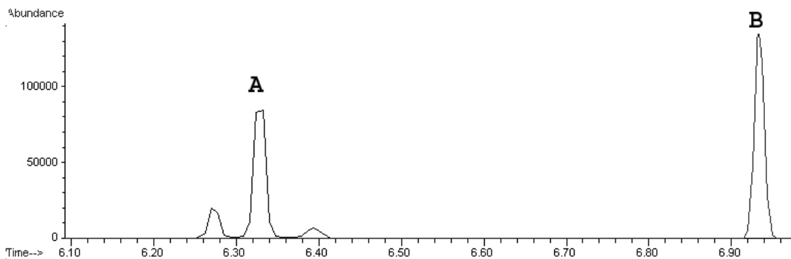
Figure 13. Gas chromatogram for confirmation of valproic acid (A) with internal standard (B).
