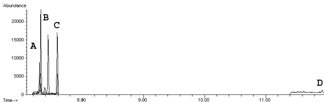
Figure 6. Gas chromatogram for confirmation of butalbital (B), amobarbital (C), and meprobamate (D) with internal standard (A).
