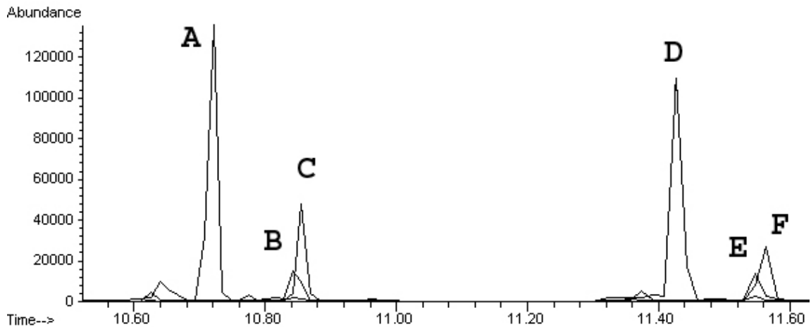
Figure 8. Gas chromatogram for confirmation of amitriptyline (A), imipramine (C), nortriptyline (D), and desipramine (F) with internal standards (B and E).
