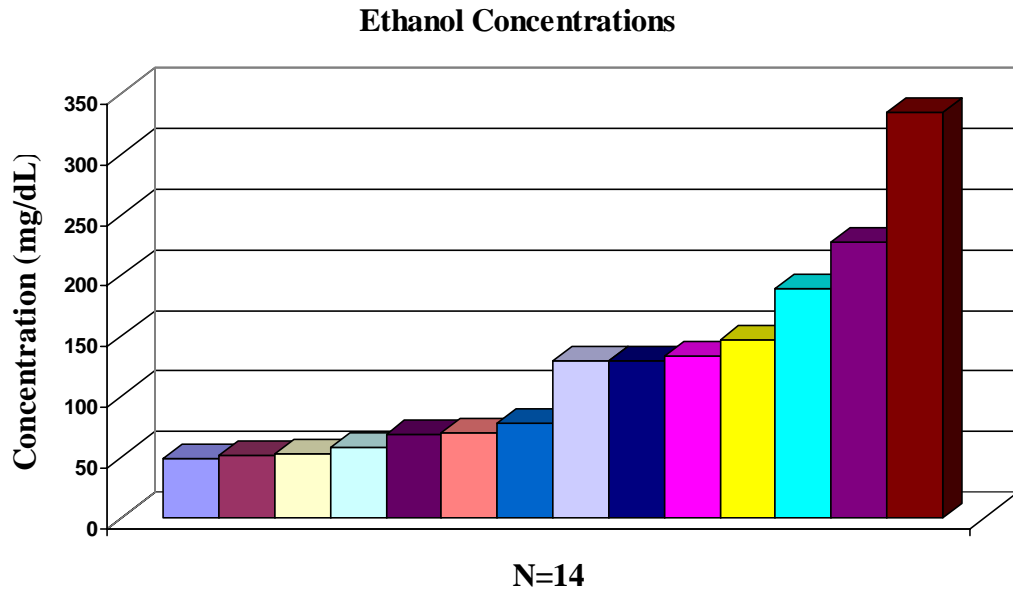
Figure 20. Concentration range for all samples (N=14) that were positive for ethanol.
