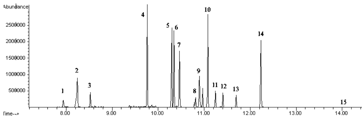
Figure 4. Representative chromatogram for control B. 1, norfluoxetine; 2, norketamine; 3, meprobamate; 4, imipramine; 5, scopolamine; 6, nortriptyline; 7, desipramine; 8, hydrocodone; 9, hydromorphone; 10, sertraline; 11, oxycodone; 12, paroxetine; 13, 7-aminoflunitrazepam; 14, zolpidem; and 15, \alpha -hydroxytriazolam.
