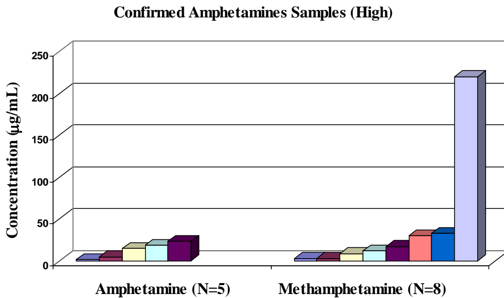
Figure 29. High concentrations for samples that were positive for either amphetamine or methamphetamine.
