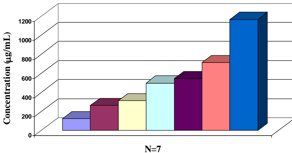
Confirmed Benzoyllecgonine Concentrations (High)
