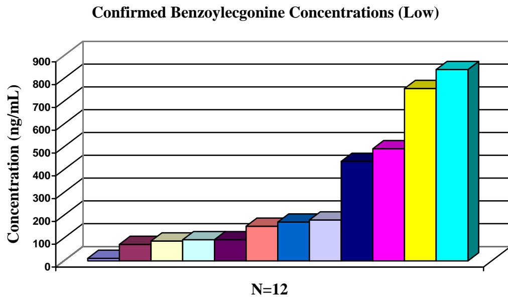
Figure 21. Low concentrations for samples (N=12) that were positive for the metabolite of cocaine (benzoyllecgonine).
