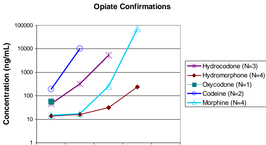
Figure 26. Concentrations of samples positive for one of the opiates being analyzed.
