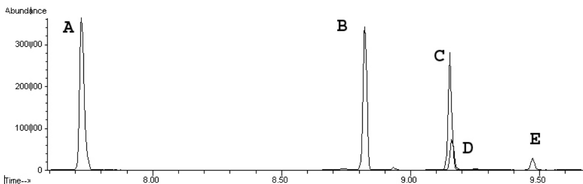
Figure 14. Gas chromatogram for confirmation of cocaine (A), codeine (B), sertraline (C), and chlordiazepoxide (D) with internal standard (E).
