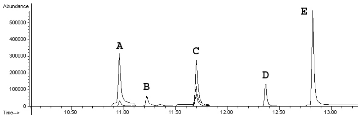
Figure 10. Gas chromatogram for confirmation of diphenhydramine (A), doxylamine (B), chlorpheniramine (C), dextromethorphan (D), and cyclobenzaprine (E).
