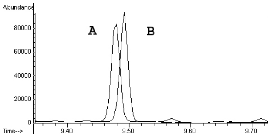
Figure 11. Gas chromatogram for confirmation of paroxetine (B) with internal standard (A).
