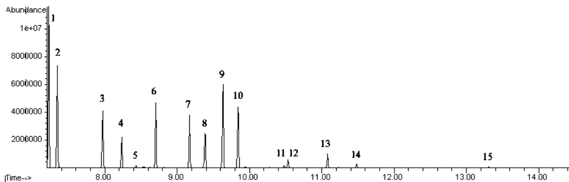
Figure 3. Representative chromatogram for control A. 1, butalbital; 2, amobarbital; 3, diphenhydramine; 4, doxylamine; 5, carisoprodol; 6, chlorpheniramine; 7, clonidine; 8, dextromethorphan; 9, amitriptyline; 10, cyclobenzaprine; 11, desmethyldoxepin; 12, citalopram; 13, chlordiazepoxide; 14, 7-aminoclonazepam; and 15, \alpha -hydroxyalprazolam.
