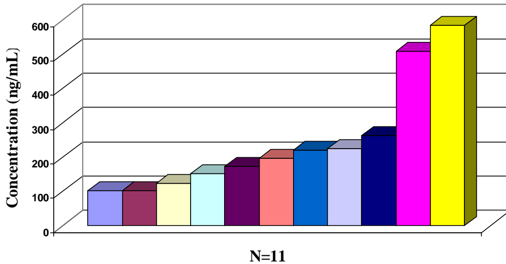
Figure 25. High concentrations for samples (N=11) that were positive for the metabolite of THC (carboxy-THC).
