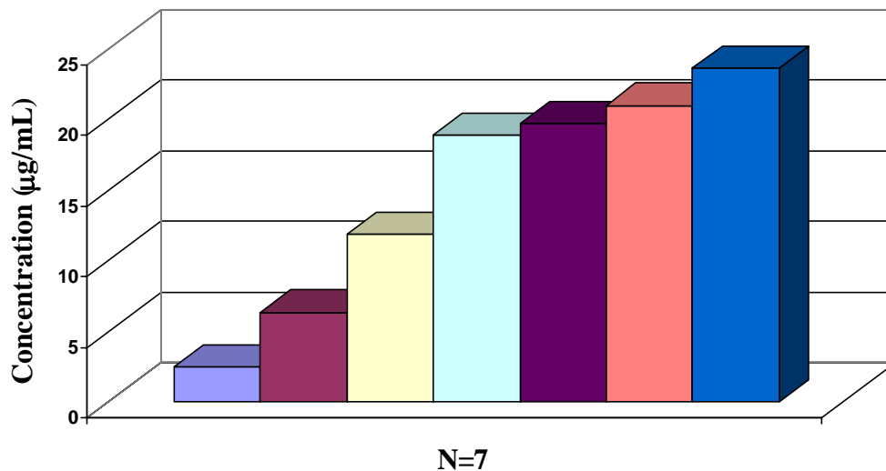
Figure 22. Middle concentrations for samples (N=7) that were positive for the metabolite of cocaine (benzoyllecgonine).
