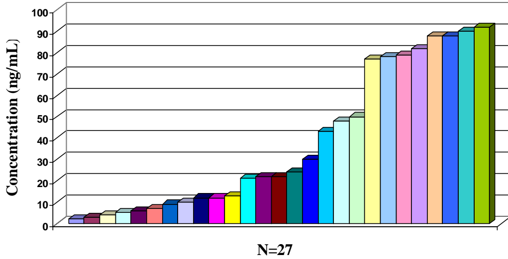
Figure 24. Low concentrations for samples (N=27) that were positive for the metabolite of THC (carboxy-THC).
