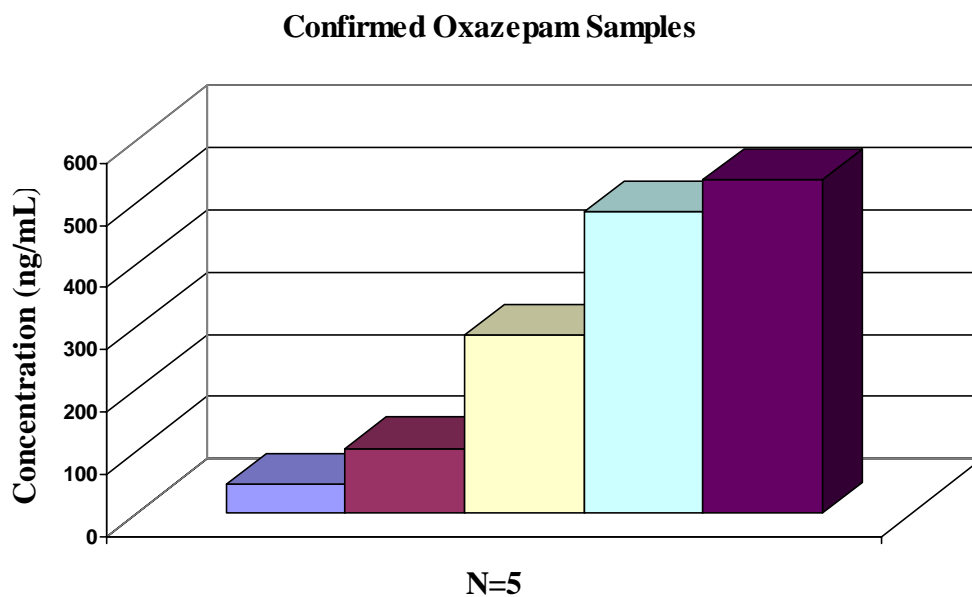
Figure 27. Concentrations for samples (N=5) that were positive for the common metabolite of most benzodiazepines (oxazepam).
