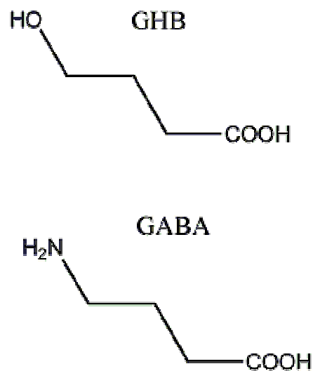
Figure 1. Structural similarities of GHB and GABA.
