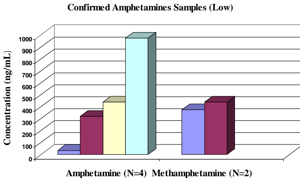
Figure 28. Low concentrations for samples that were positive for either amphetamine or methamphetamine.
