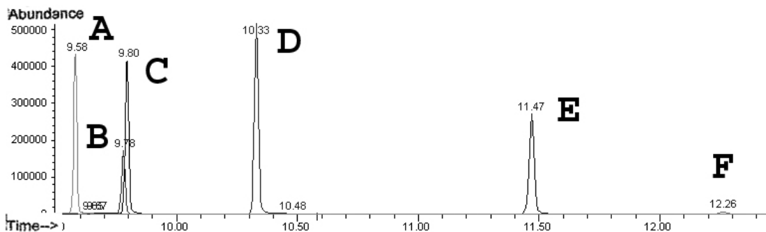
Figure 7. Gas chromatogram for confirmation of \alpha -hydroxyalprazolam (E), \alpha -hydroxytriazolam (F), 7-aminoclonazepam (A), 7-aminoflunitrazepam (C), and zolpidem (D) with internal standard (B).
