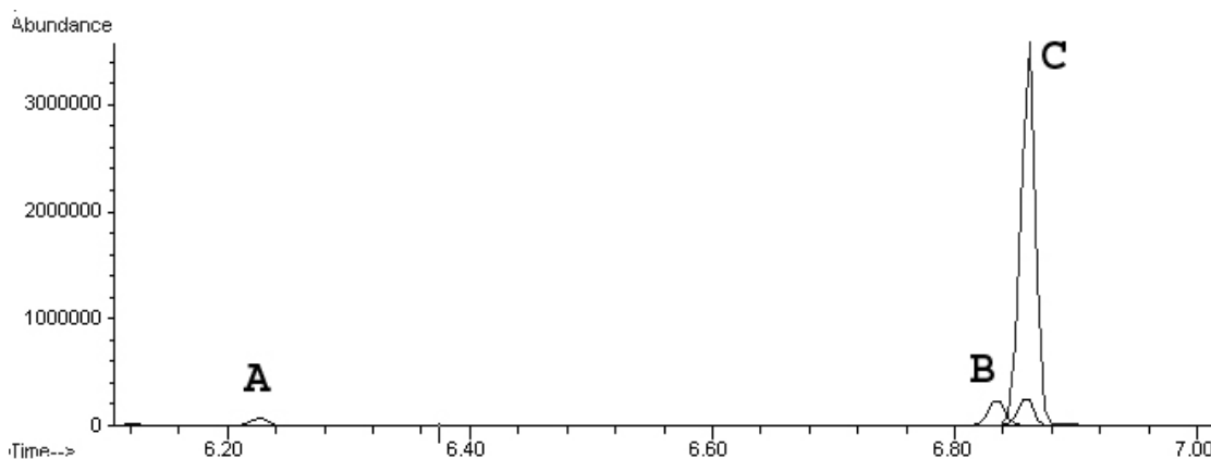
Figure 12. Gas chromatogram for screening/confirmation of GHB (C) and screening of valproic acid (A) with internal standard (B).
